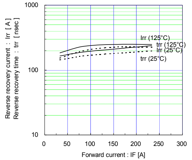
Reverse recovery characteristics (typ.) Vcc=900V, VGE=±15V, Rg=3.3Ω
