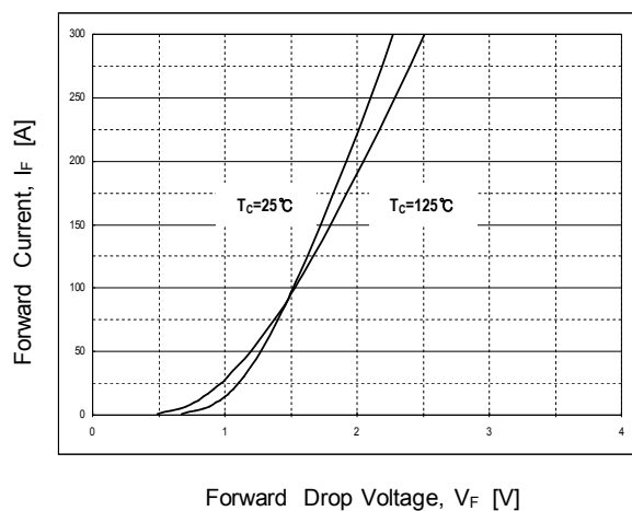
Fig 12. Forward characteristics
