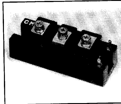
CM150E3Y-12E Chopper IGBTMOD™ E-Series Module 150 Amperes/600 Volts
