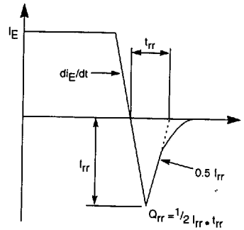
t_{rr}, Q_{rr} WAVEFORMS
