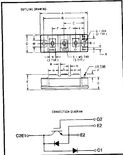
CM150E3Y-12E Outline Drawing
