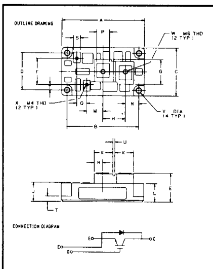
CM300HA-12E Outline Drawing
