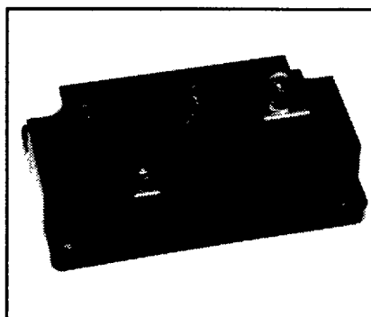
CM300HA-12E Single IGBTMOD™ E-Series Module 300 Amperes/600 Volts
