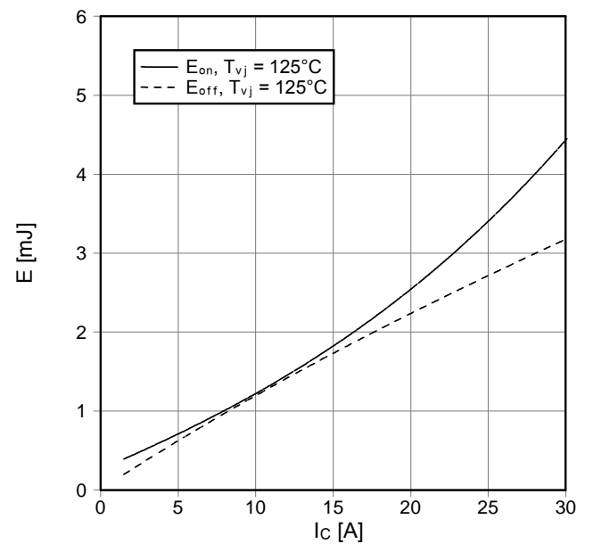
Schaltverluste IGBT-Wechselr. (typisch) switching losses IGBT-inverter (typical) E_{on} = f(I_C) , E_{off} = f(I_C) V_{GE} = \pm 15\text{ V} , R_{Gon} = 75\ \Omega , R_{Goff} = 75\ \Omega , V_{CE} = 600\text{ V}
