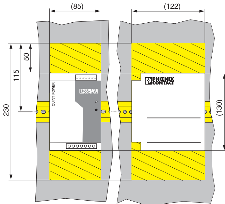
Figure 4 Mounting position (dimensions in mm)
