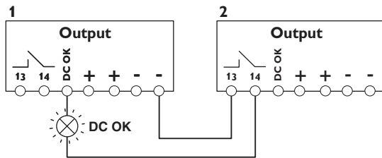
Figure 12 Signal loop
