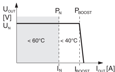
Figure 13 Output characteristic curve
