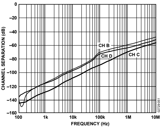
Figure 56. Channel Separation
