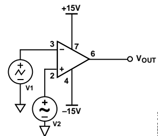
Figure 53. Pulse-Width Modulator
